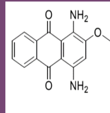
solvent violet 47 (violett)
